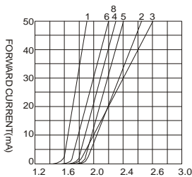
FORWARD VOLTAGE (Vf) FORWARD CURRENT VS. FORWARD VOLTAGE
